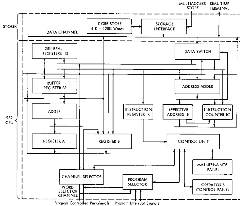
Systemblockschema
